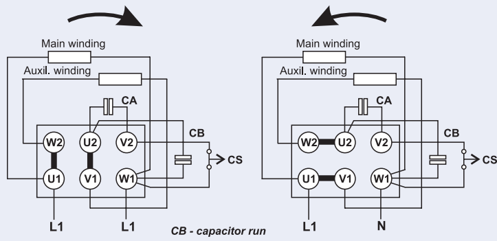
2. With capacitors start / run
